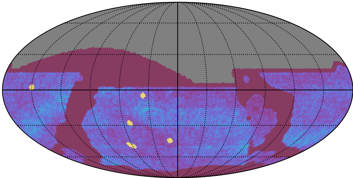
too_ignore_100_4v3.4_10yrs All sky all bands: NVisits
