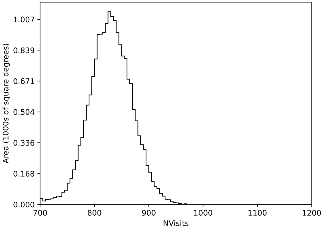
too_ignore_100_4v3.4_10yrs All sky all bands: NVisits
