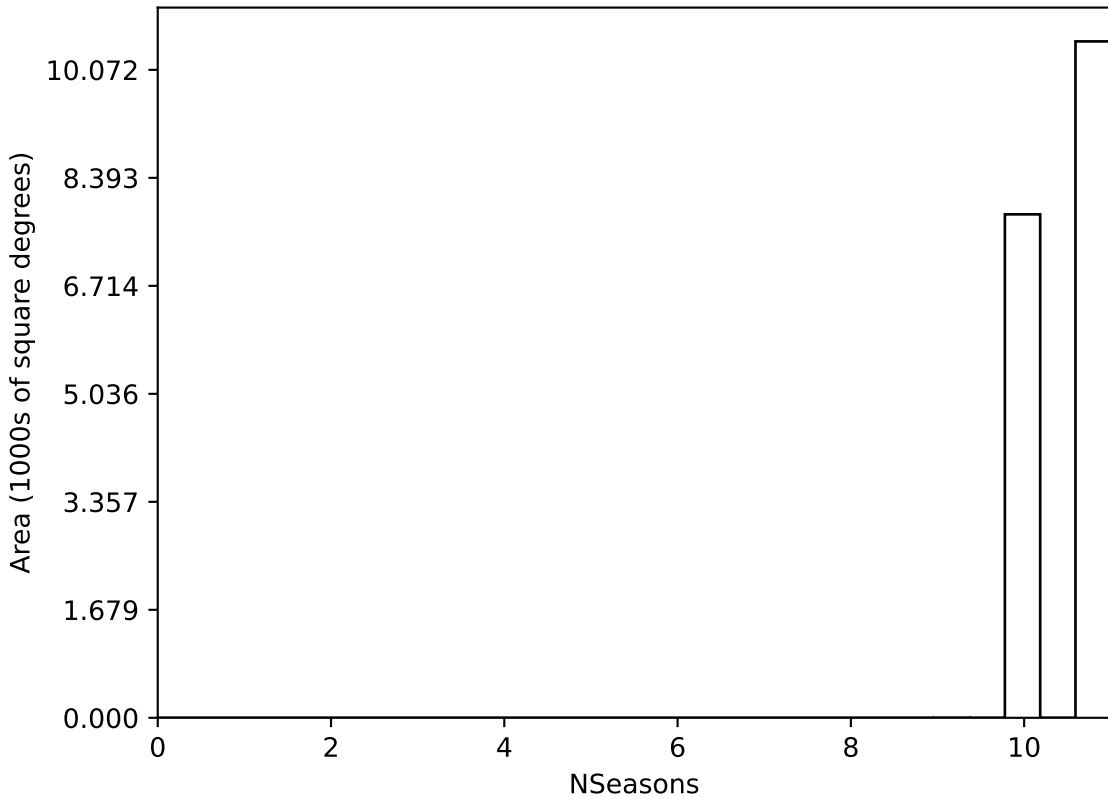
too_ignore_100_4v3.4_10yrs WFD all bands: NSeasons
