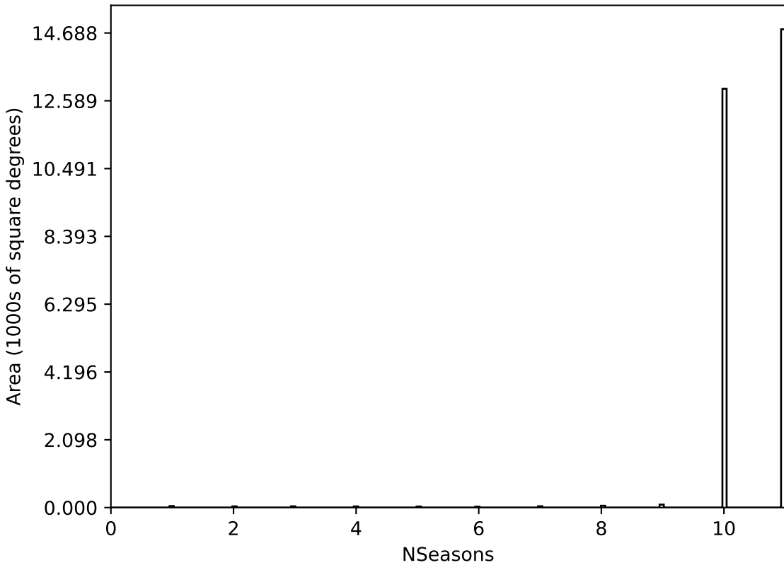
too_ignore_100_4v3.4_10yrs All sky all bands: NSeasons
