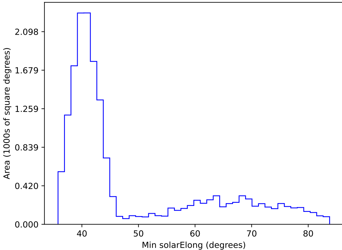
too_ignore_100_4v3.4_10yrs WFD z band: Min solarElong
