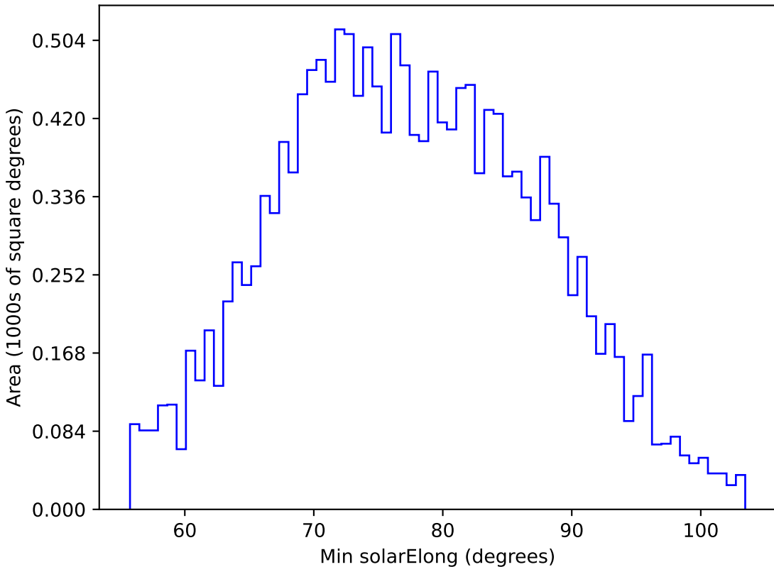
too_ignore_100_4v3.4_10yrs WFD u band: Min solarElong
