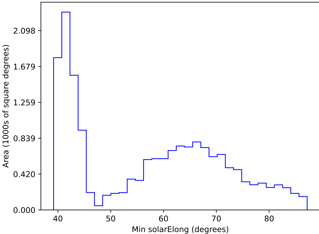
too_ignore_100_4v3.4_10yrs WFD r band: Min solarElong
