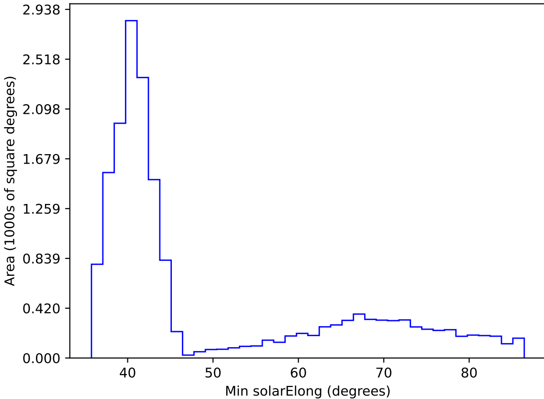
too_ignore_100_4v3.4_10yrs WFD i band: Min solarElong
