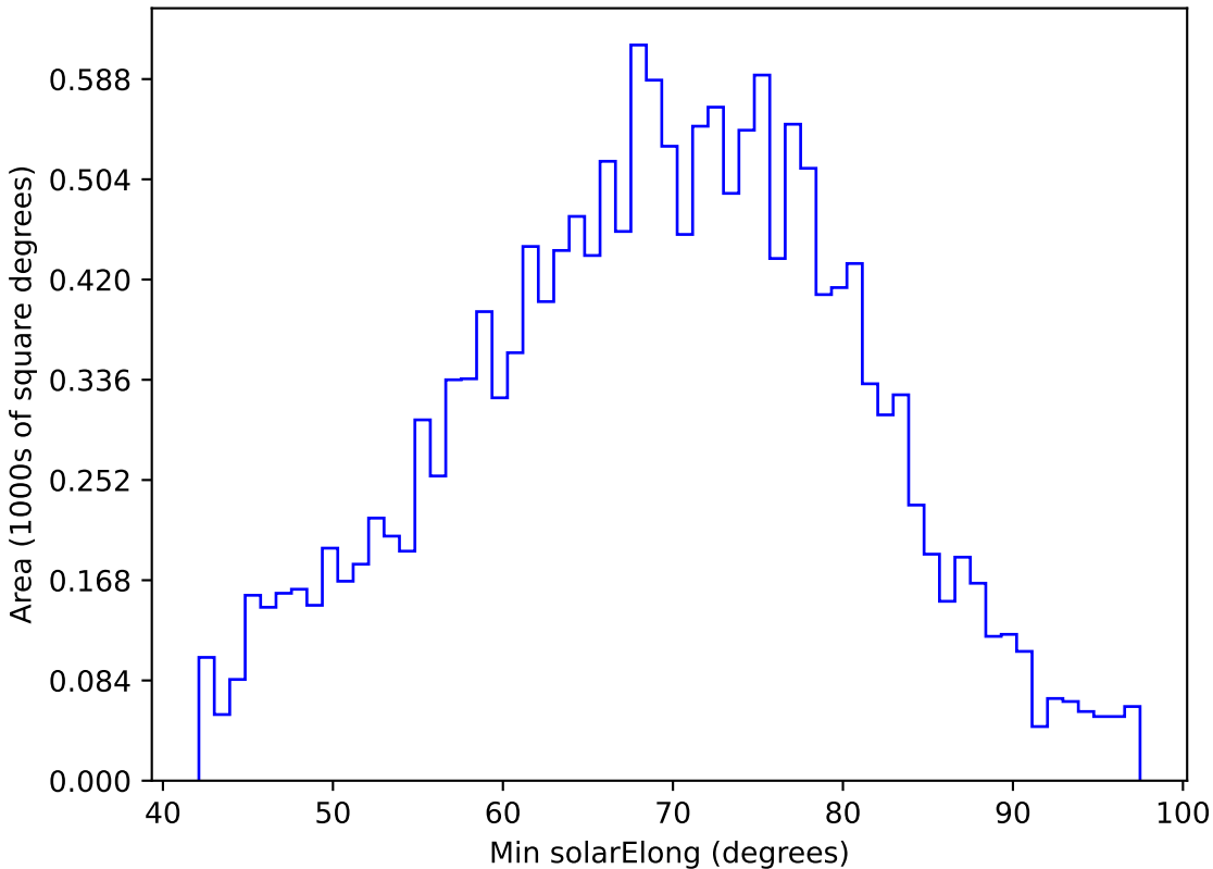
too_ignore_100_4v3.4_10yrs WFD g band: Min solarElong
