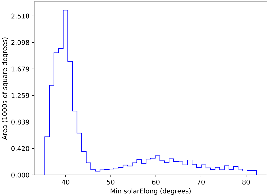
too_ignore_100_4v3.4_10yrs WFD all bands: Min solarElong
