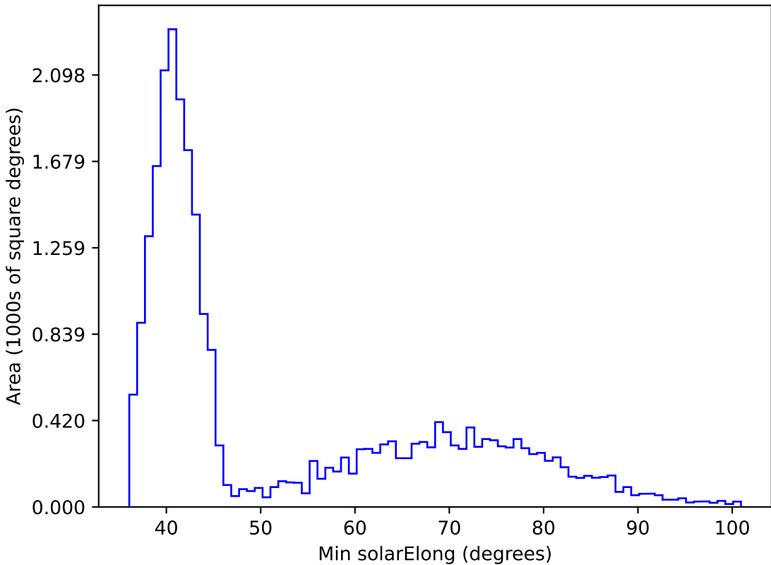
too_ignore_100_4v3.4_10yrs All sky z band: Min solarElong
