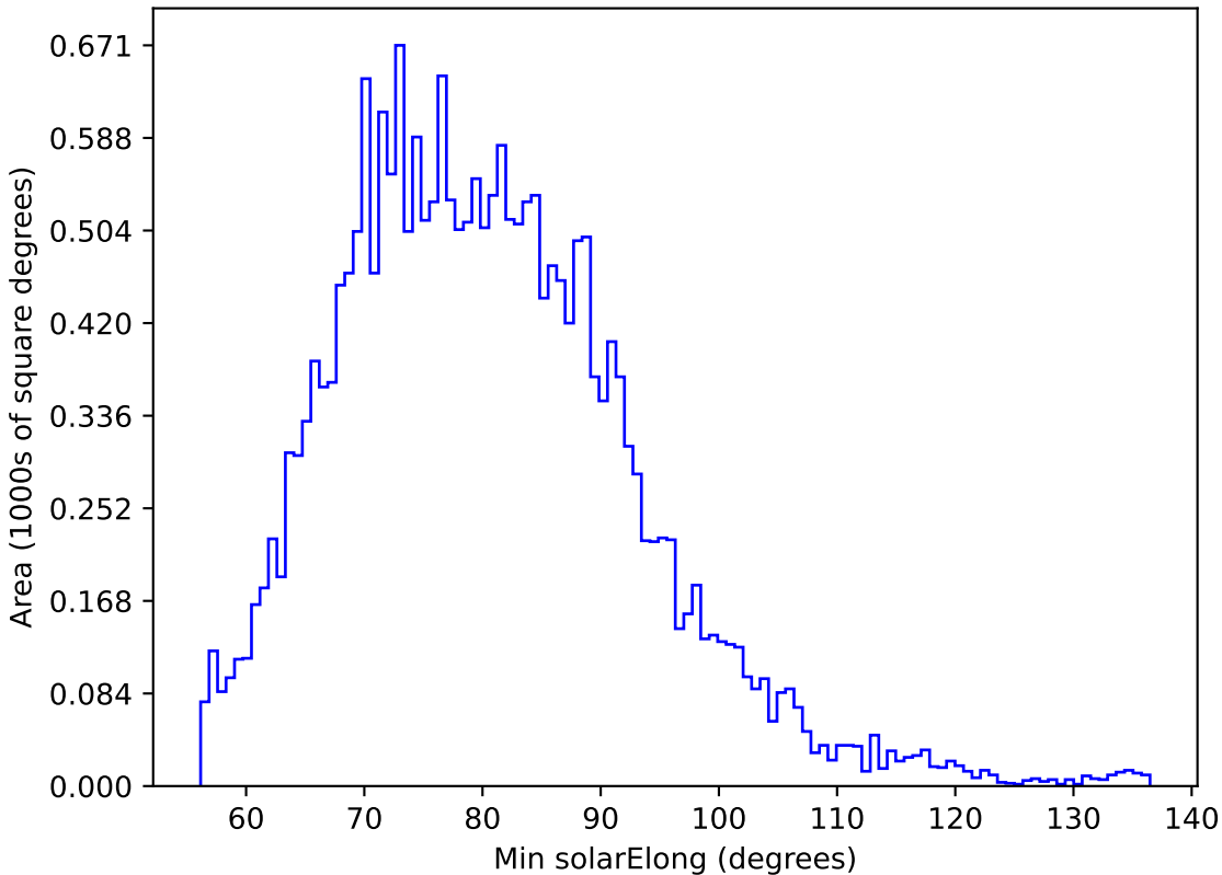
too_ignore_100_4v3.4_10yrs All sky u band: Min solarElong
