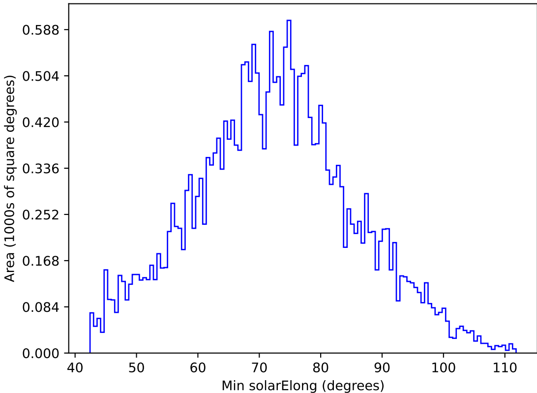
too_ignore_100_4v3.4_10yrs All sky g band: Min solarElong
