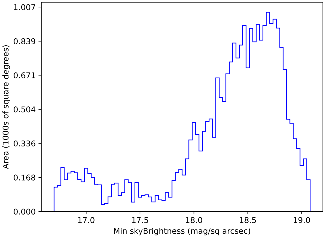
too_ignore_100_4v3.4_10yrs Yr 1 z band: Min skyBrightness
