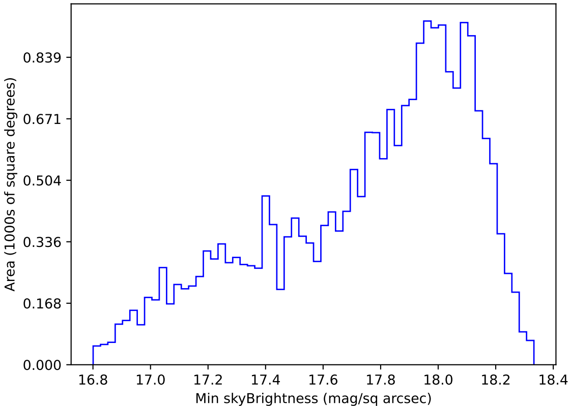
too_ignore_100_4v3.4_10yrs Yr 1 y band: Min skyBrightness
