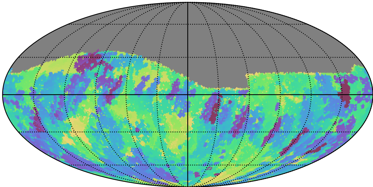
too_ignore_100_4v3.4_10yrs Yr 1 r band: Min skyBrightness
