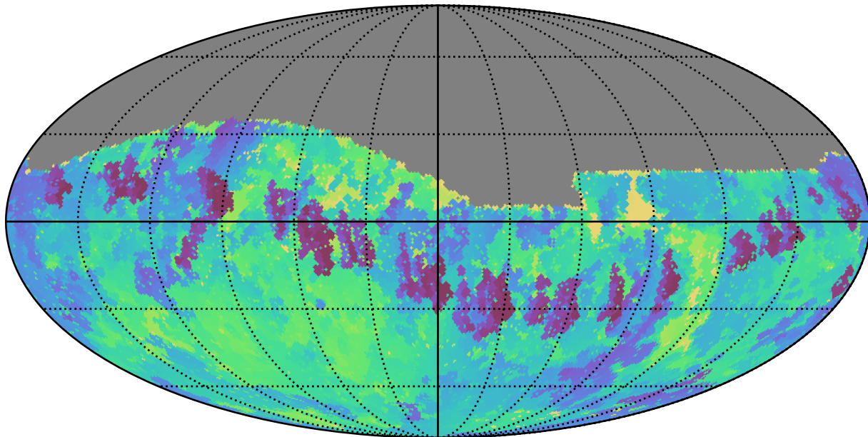
too_ignore_100_4v3.4_10yrs Yr 1 i band: Min skyBrightness
