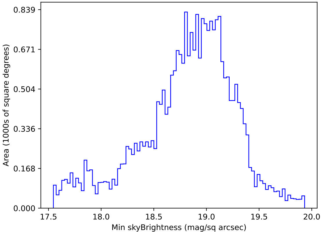
too_ignore_100_4v3.4_10yrs Yr 1 i band: Min skyBrightness
