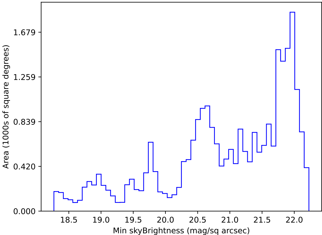
too_ignore_100_4v3.4_10yrs Yr 1 g band: Min skyBrightness
