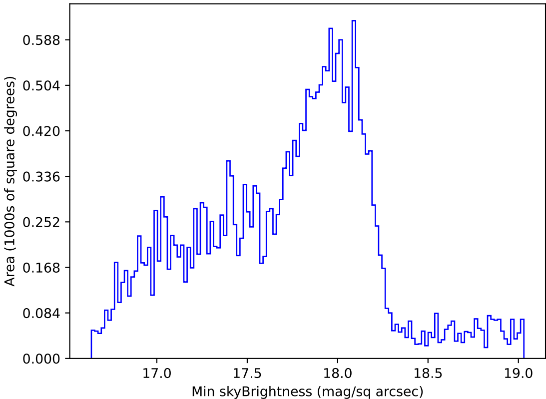
too_ignore_100_4v3.4_10yrs Yr 1 all bands: Min skyBrightness
