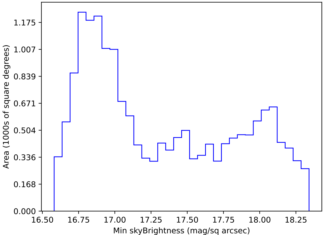
too_ignore_100_4v3.4_10yrs WFD z band: Min skyBrightness
