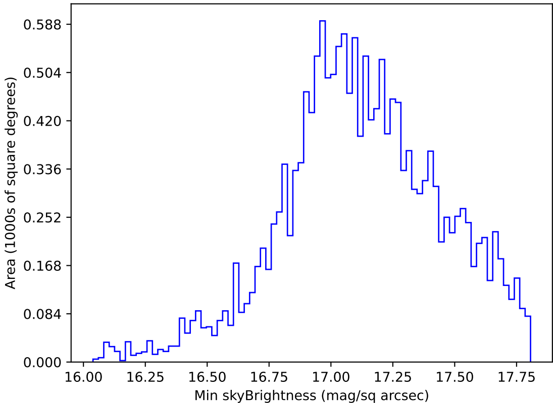
too_ignore_100_4v3.4_10yrs WFD y band: Min skyBrightness
