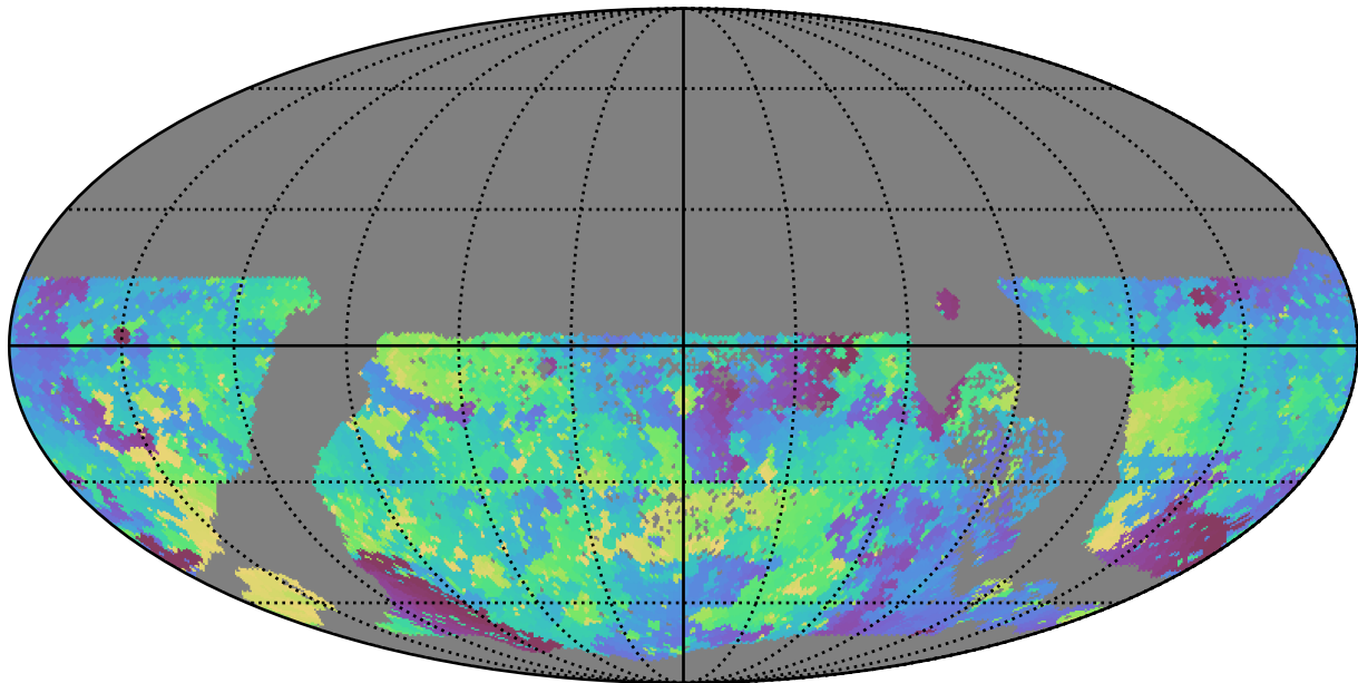
too_ignore_100_4v3.4_10yrs WFD u band: Min skyBrightness
