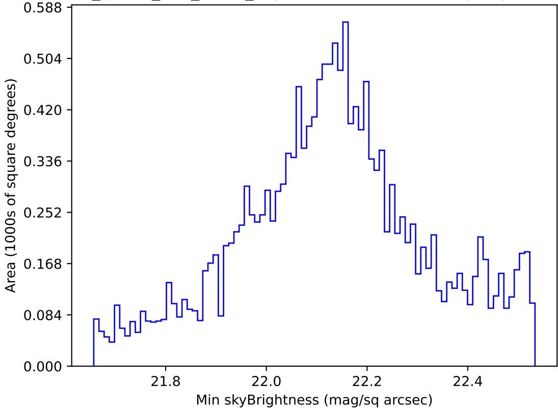
too_ignore_100_4v3.4_10yrs WFD u band: Min skyBrightness
