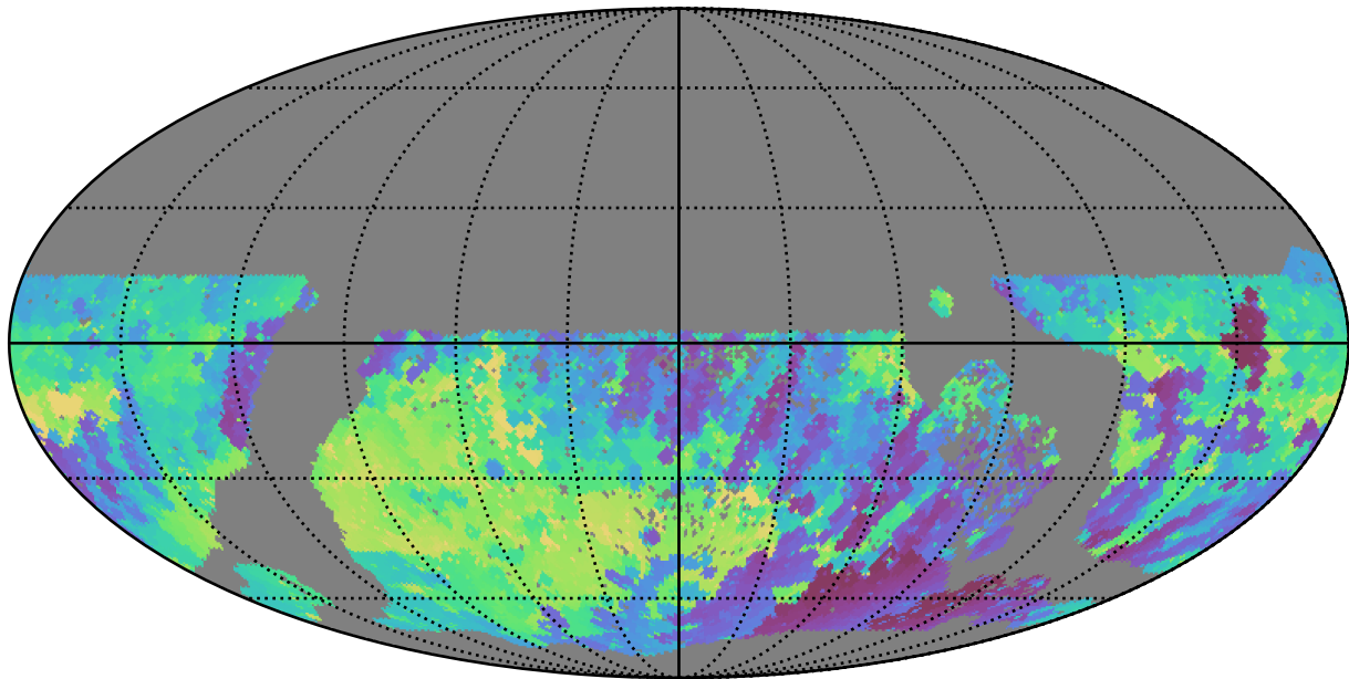
too_ignore_100_4v3.4_10yrs WFD r band: Min skyBrightness
