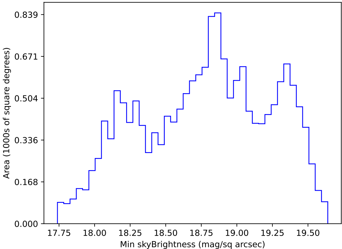
too_ignore_100_4v3.4_10yrs WFD r band: Min skyBrightness
