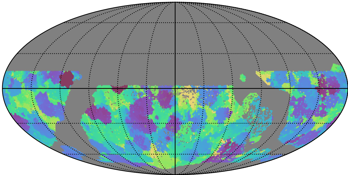
too_ignore_100_4v3.4_10yrs WFD g band: Min skyBrightness
