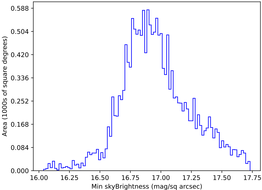
too_ignore_100_4v3.4_10yrs WFD all bands: Min skyBrightness
