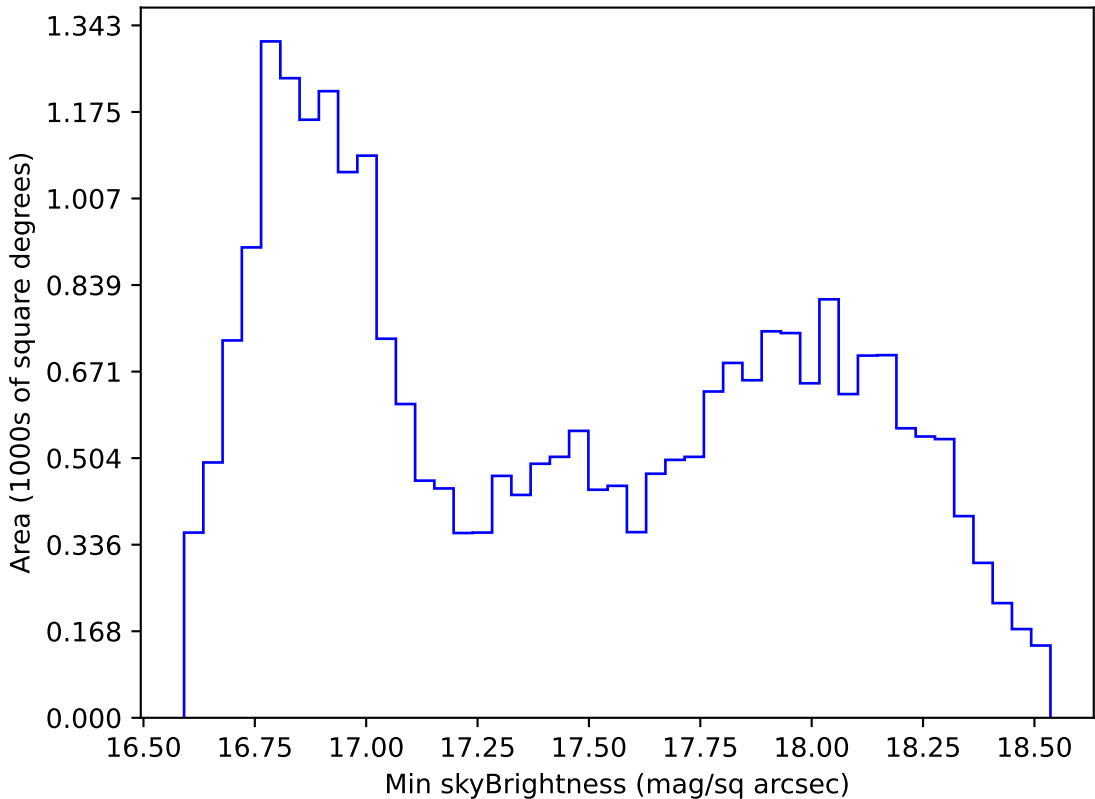
too_ignore_100_4v3.4_10yrs All sky z band: Min skyBrightness
