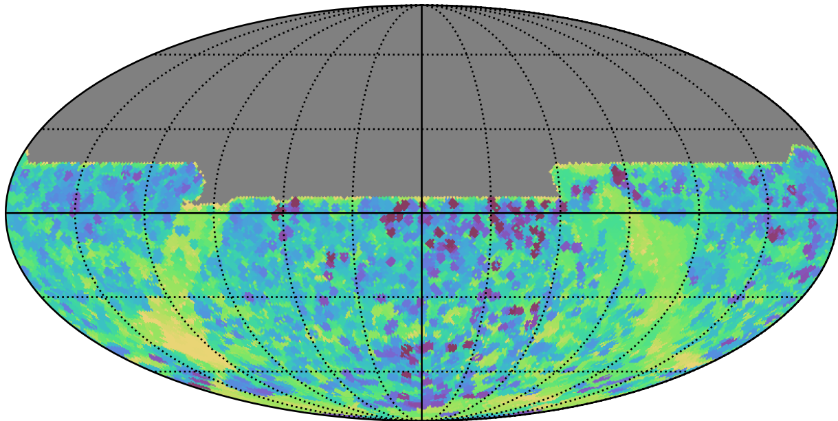
too_ignore_100_4v3.4_10yrs All sky y band: Min skyBrightness
