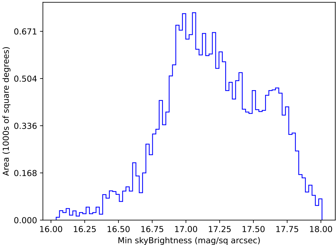
too_ignore_100_4v3.4_10yrs All sky y band: Min skyBrightness
