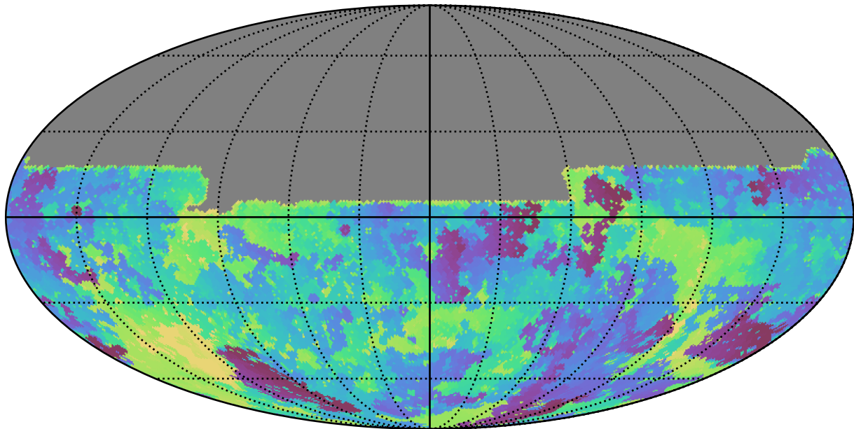
too_ignore_100_4v3.4_10yrs All sky u band: Min skyBrightness
