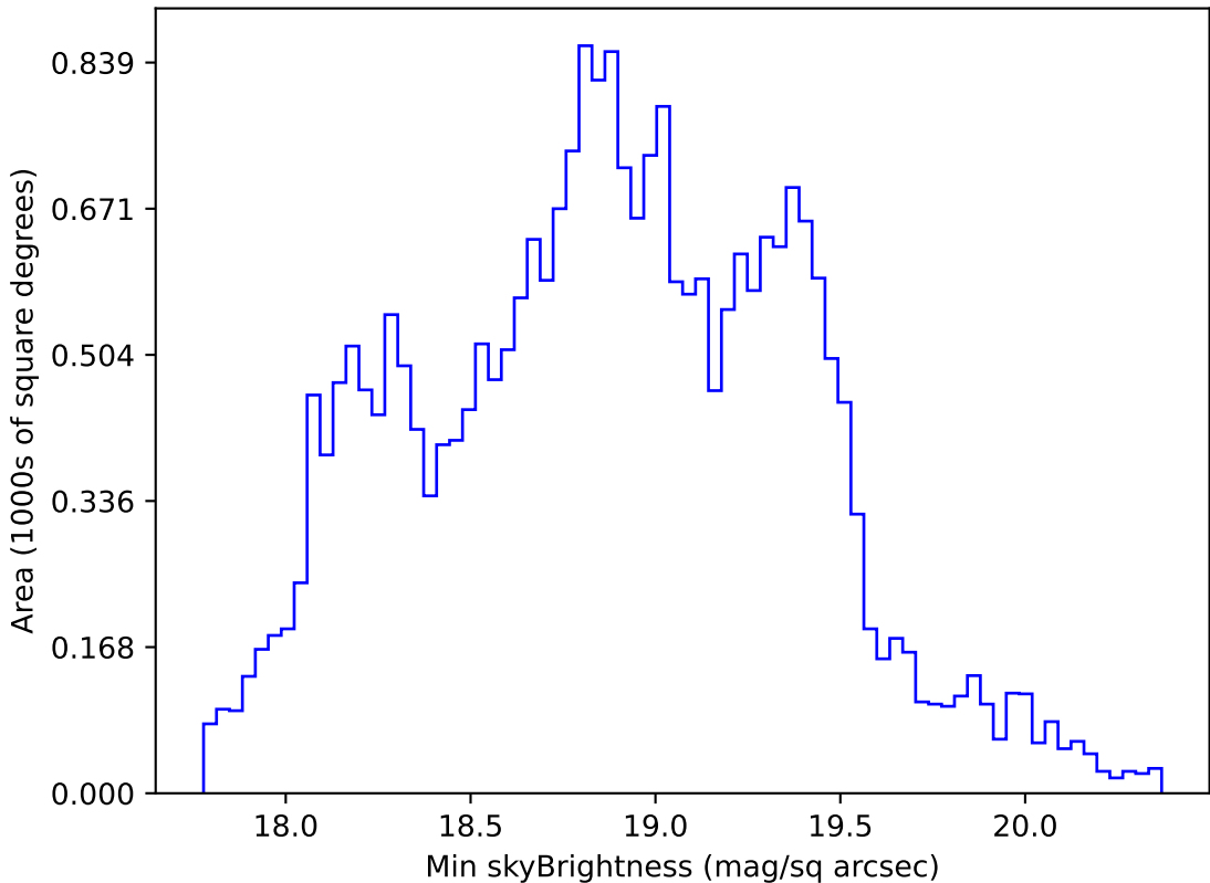
too_ignore_100_4v3.4_10yrs All sky r band: Min skyBrightness
