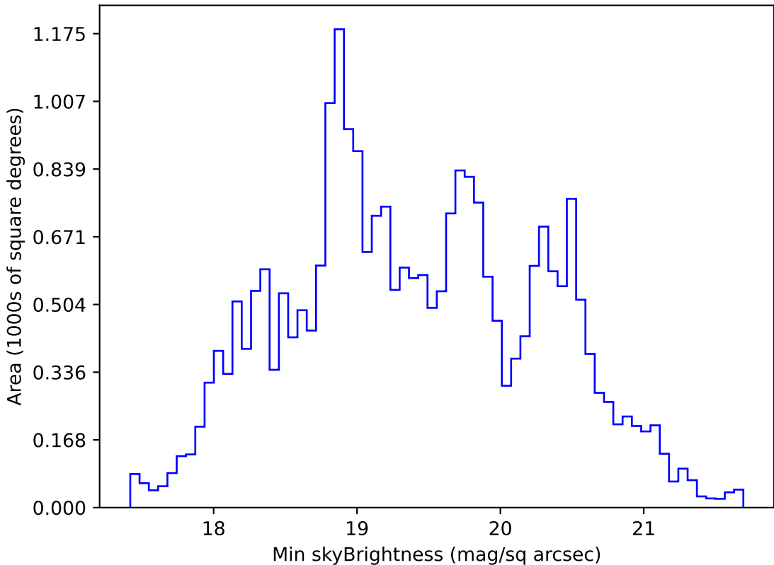
too_ignore_100_4v3.4_10yrs All sky g band: Min skyBrightness
