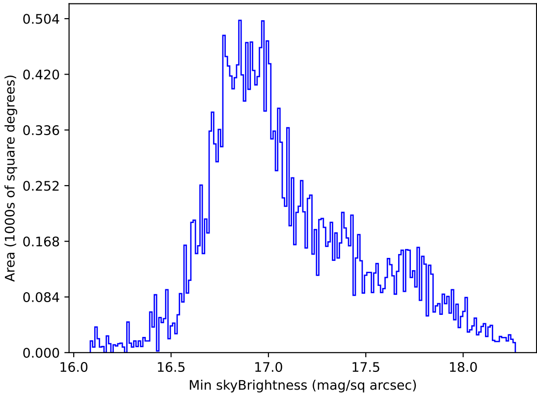
too_ignore_100_4v3.4_10yrs All sky all bands: Min skyBrightness
