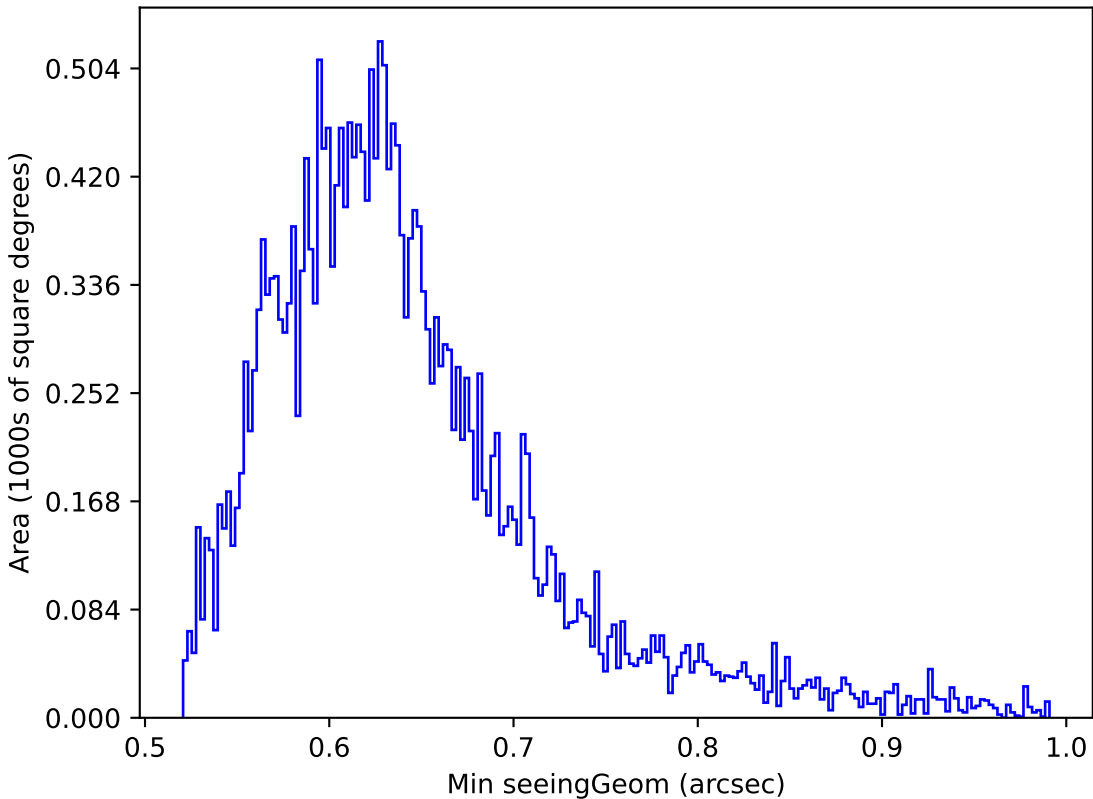
too_ignore_100_4v3.4_10yrs Yr 1 z band: Min seeingGeom
