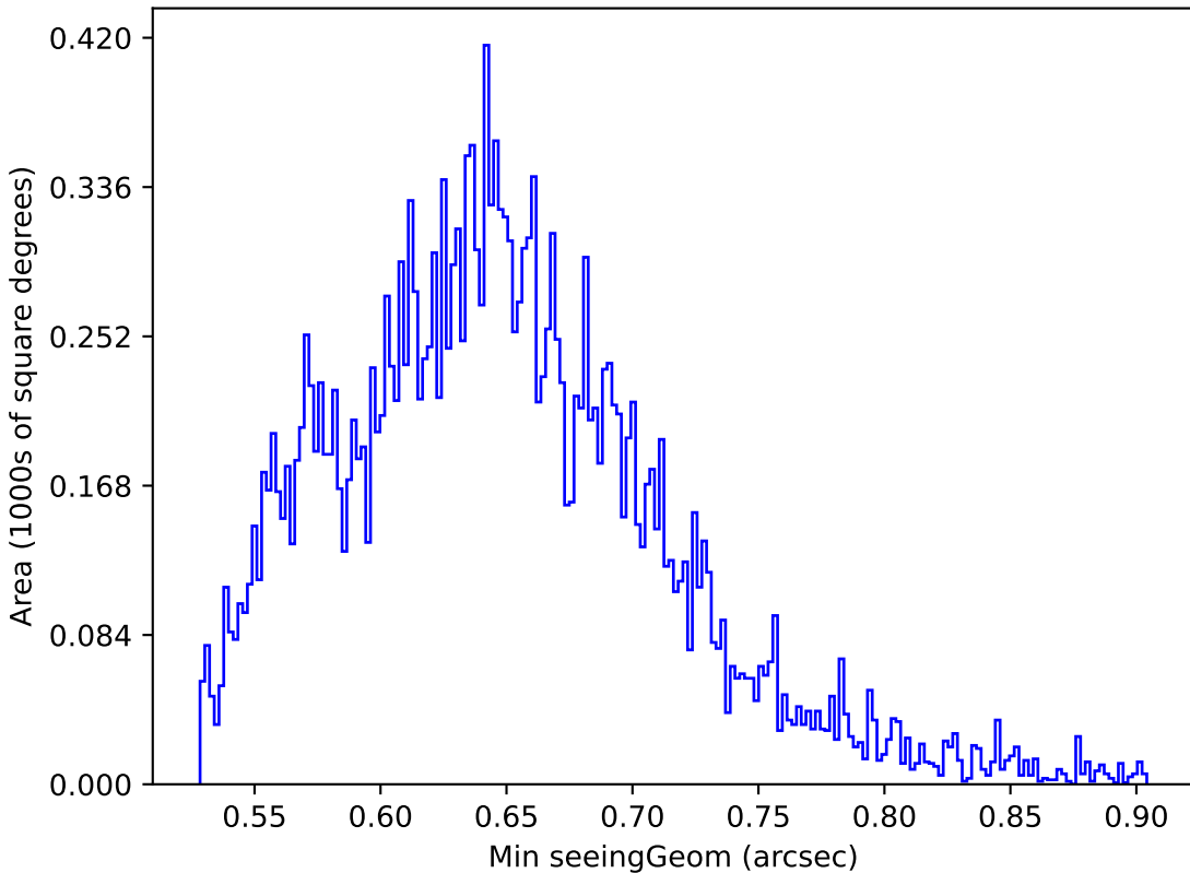
too_ignore_100_4v3.4_10yrs Yr 1 y band: Min seeingGeom
