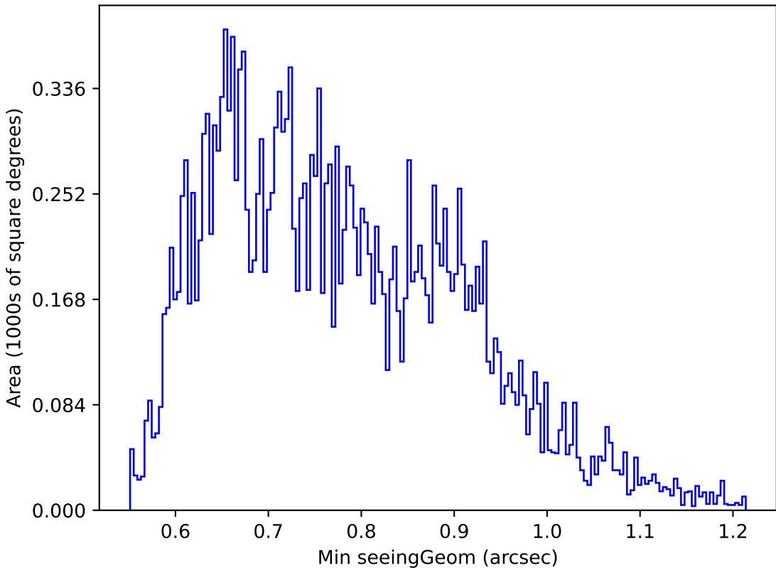
too_ignore_100_4v3.4_10yrs Yr 1 u band: Min seeingGeom
