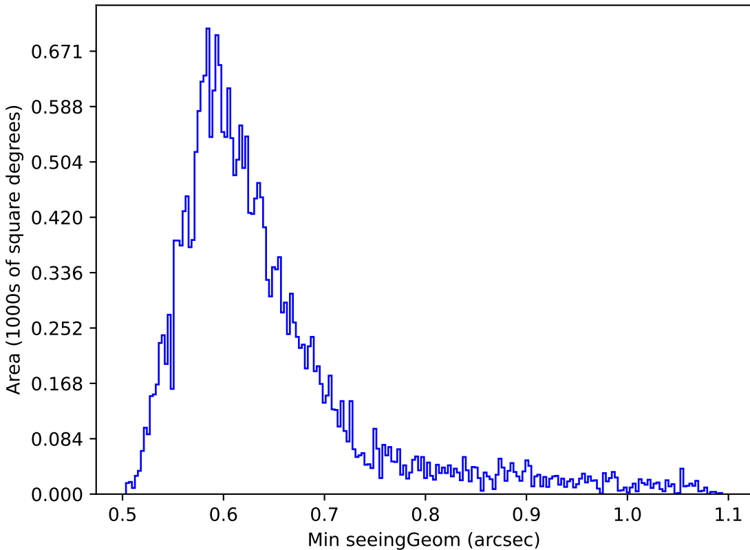
too_ignore_100_4v3.4_10yrs Yr 1 r band: Min seeingGeom
