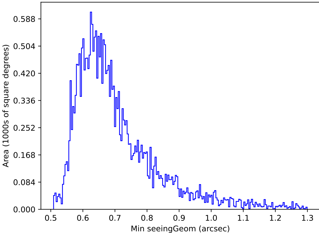
too_ignore_100_4v3.4_10yrs Yr 1 g band: Min seeingGeom
