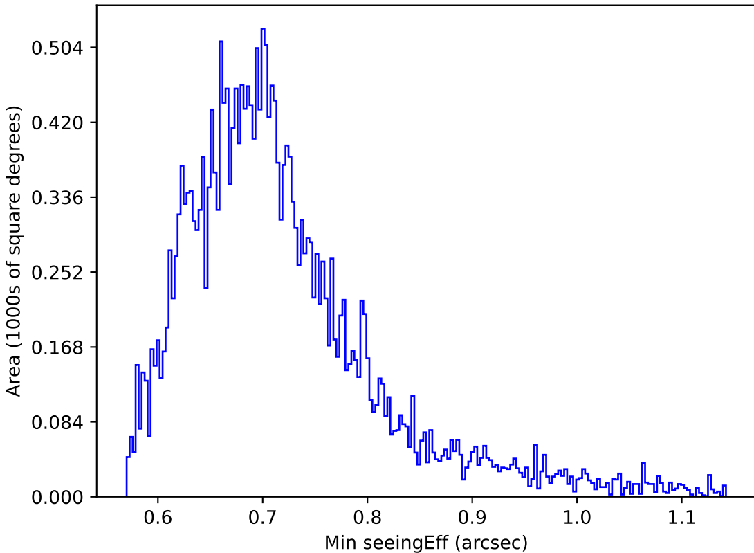
too_ignore_100_4v3.4_10yrs Yr 1 z band: Min seeingEff
