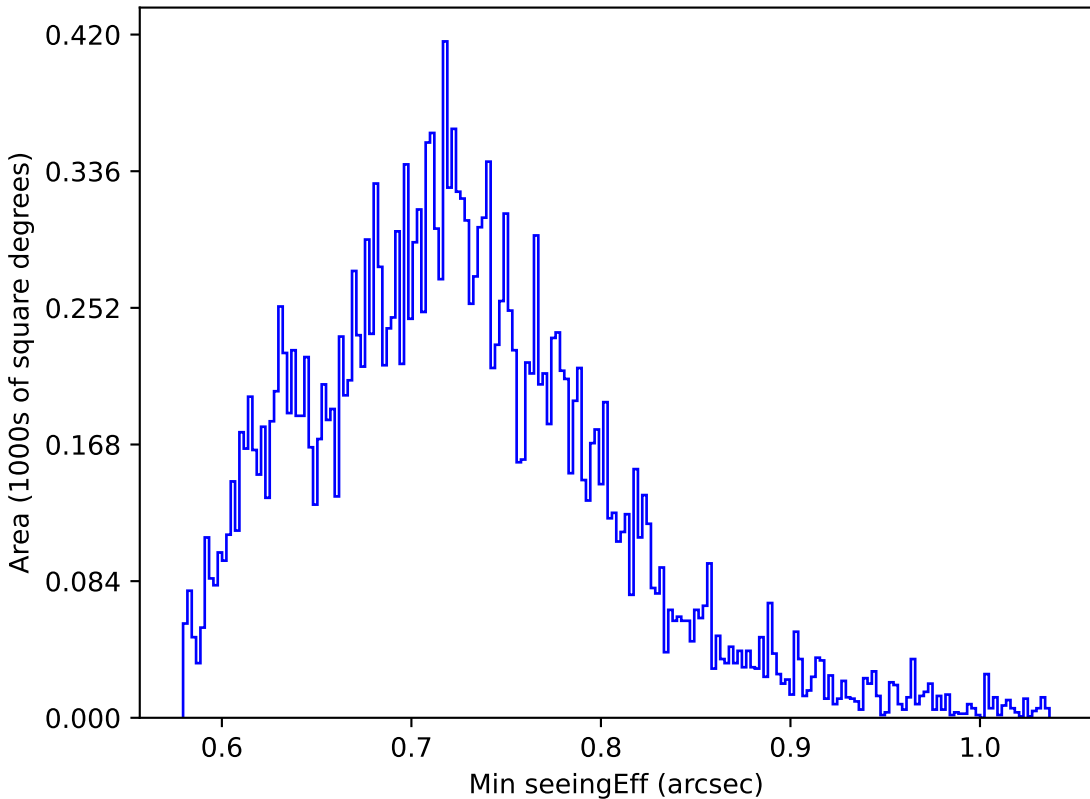
too_ignore_100_4v3.4_10yrs Yr 1 y band: Min seeingEff
