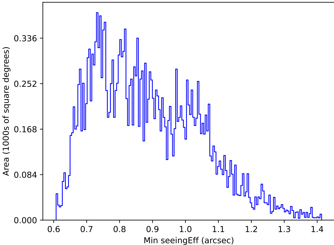
too_ignore_100_4v3.4_10yrs Yr 1 u band: Min seeingEff
