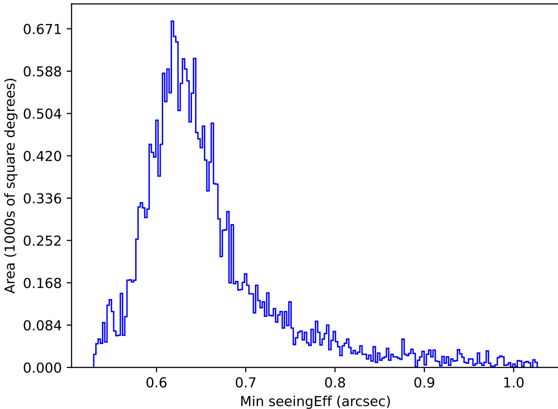
too_ignore_100_4v3.4_10yrs Yr 1 all bands: Min seeingEff
