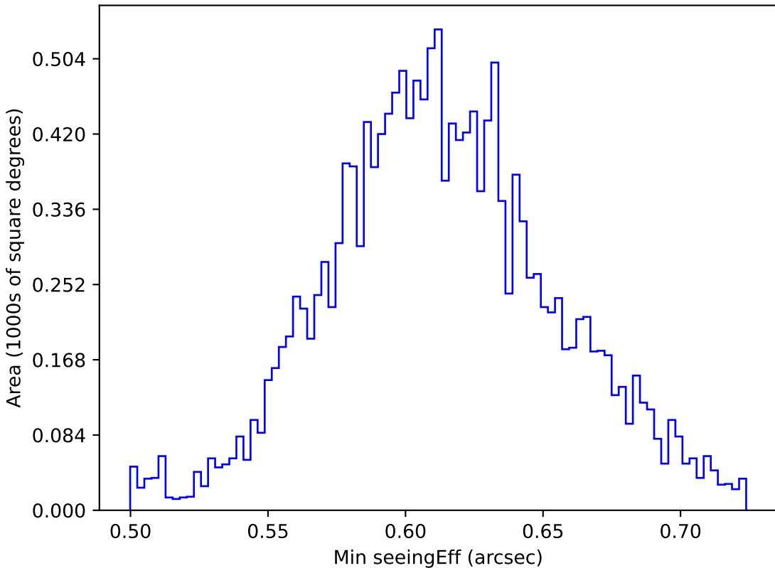
too_ignore_100_4v3.4_10yrs WFD z band: Min seeingEff
