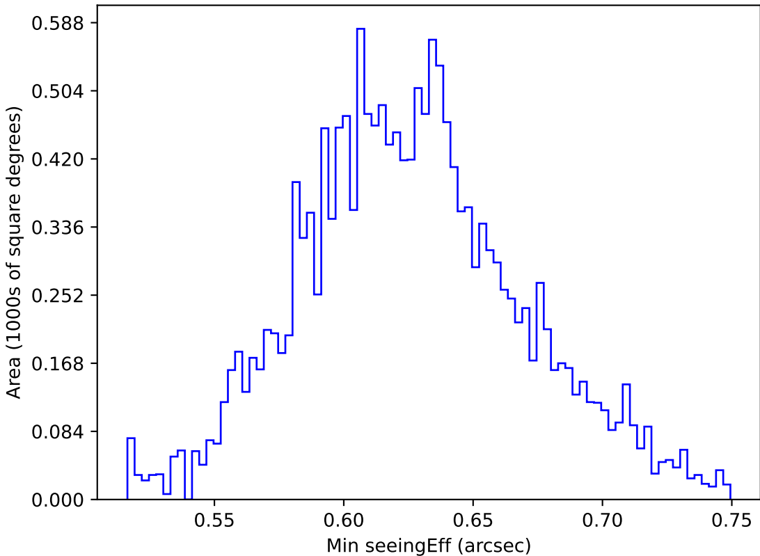
too_ignore_100_4v3.4_10yrs WFD y band: Min seeingEff
