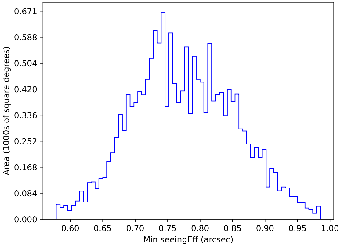
too_ignore_100_4v3.4_10yrs WFD u band: Min seeingEff
