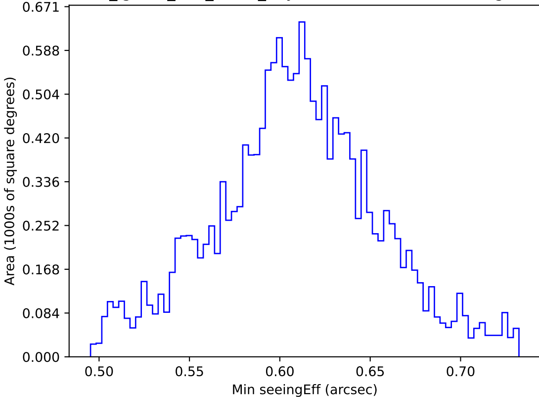
too_ignore_100_4v3.4_10yrs WFD r band: Min seeingEff
