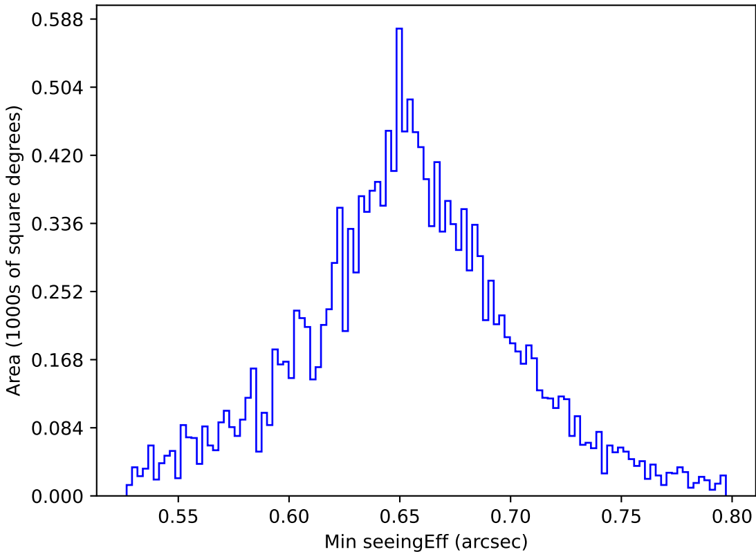
too_ignore_100_4v3.4_10yrs WFD g band: Min seeingEff
