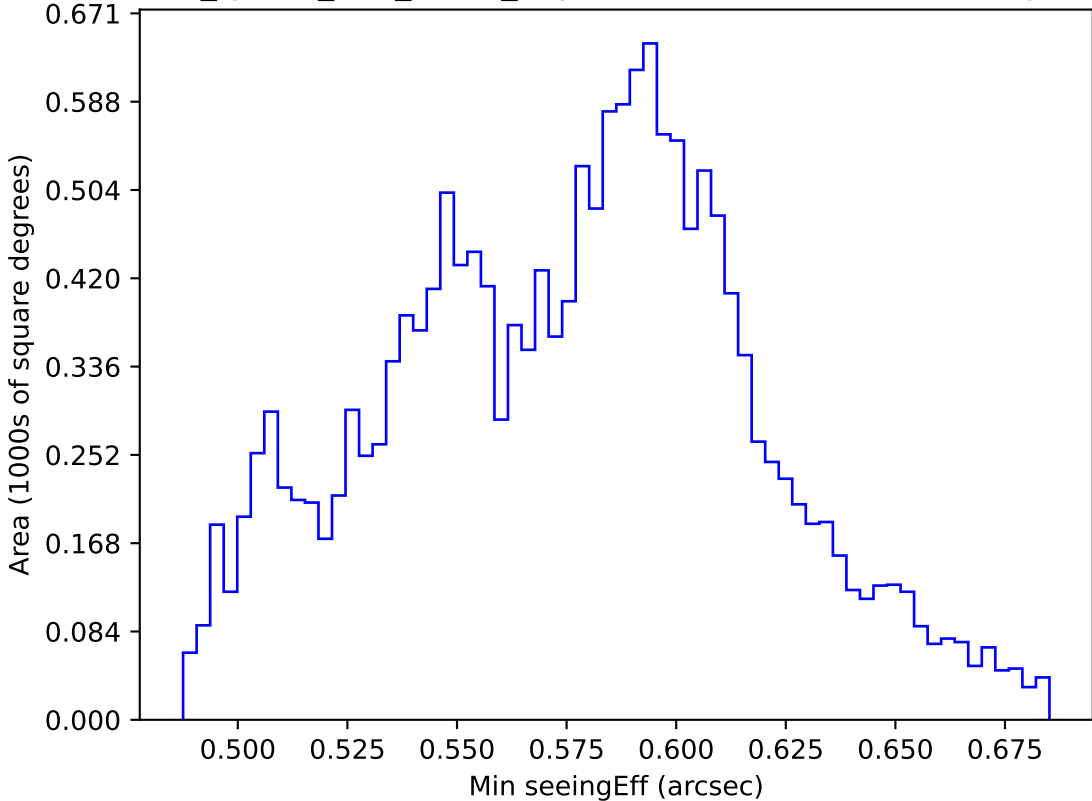
too_ignore_100_4v3.4_10yrs WFD all bands: Min seeingEff
